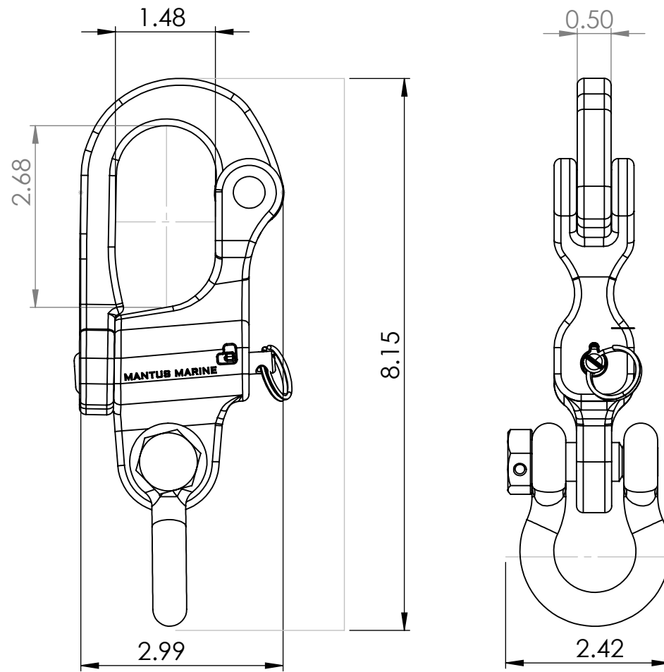
Mooring Snap Shackle 1/2 Inch, Duplex Stainless Steel
