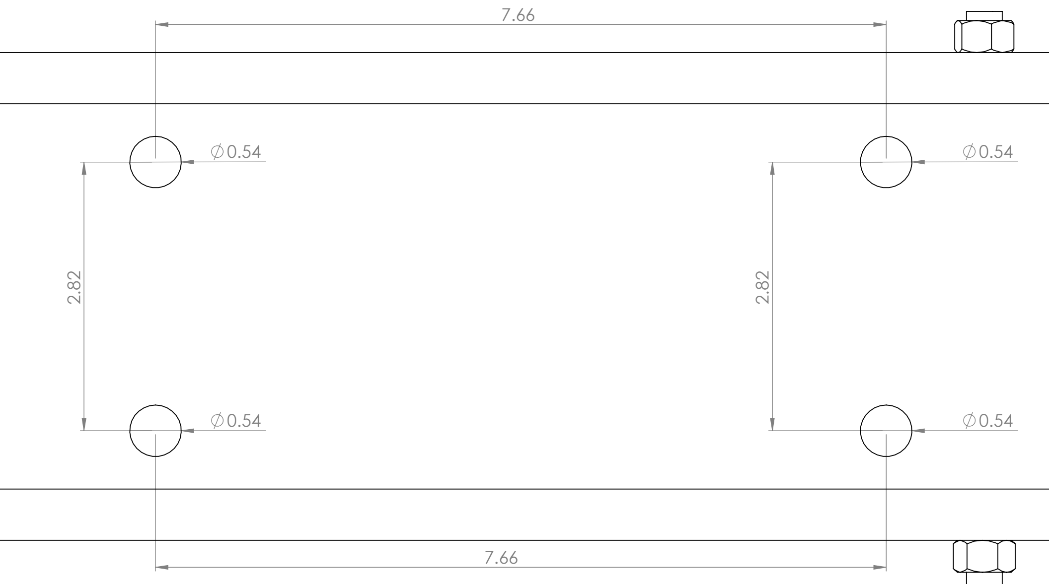
BR3 BOW ROLLER HOLE PATTERN
