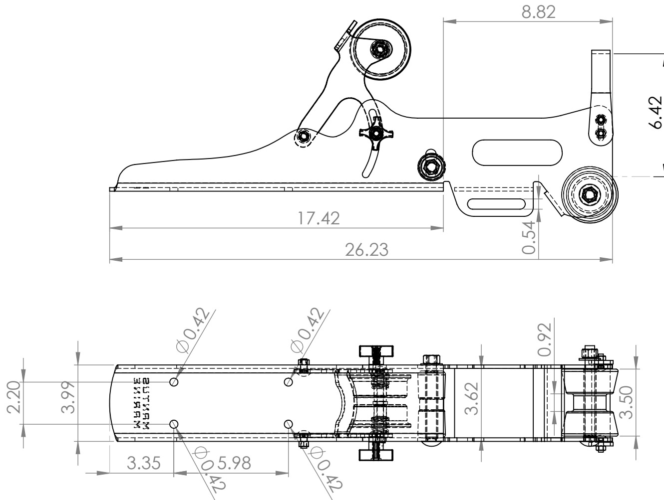
BR2 Bow Roller Dimensions
