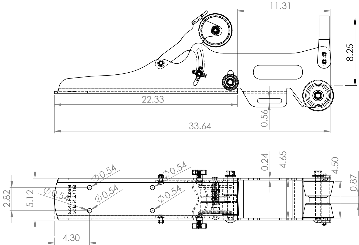
BR3 Bow Roller Dimensions
