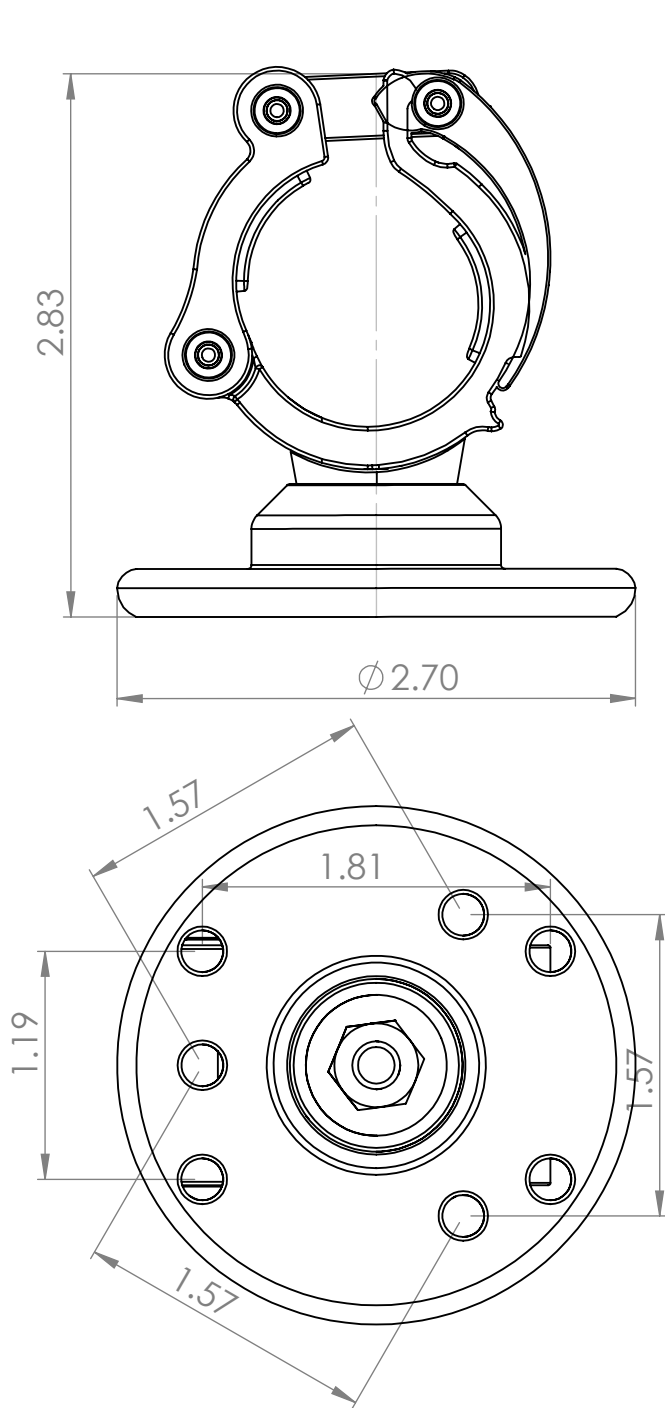
1 1/4" Inch Rail Clamp with Mounting Plate (Fits 1 1/8" and 1 1/4")
