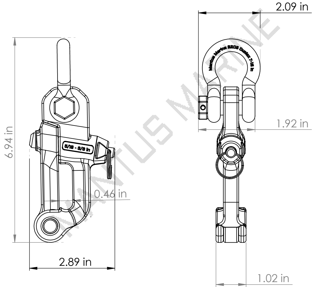
M3 CH2 Chain Hook for (5/16"/ 8mm - 3/8" /10mm chain)
