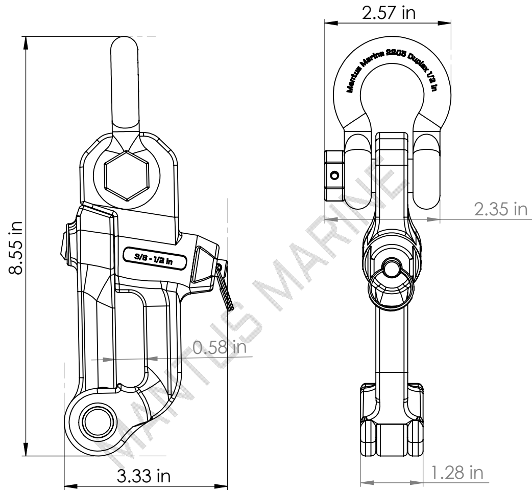
M3 CH3 Chain Hook for (3/8"/10mm to 1/2"/12mm chain)
